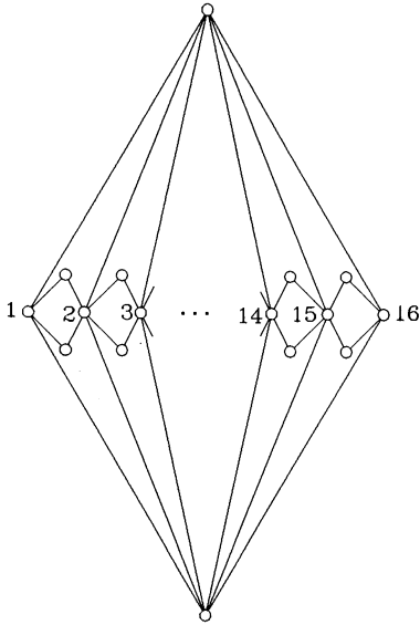
Figure 1: Four-page planar ordered set.
